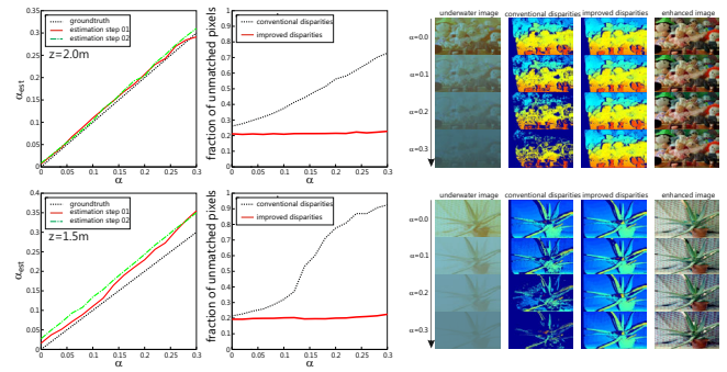
Fig. 6. Improved stereo results for decreasing visibility. Left column shows the estimated mean attenuation coefficient for decreasing visibility \alpha = 0 - 0.3 at depth z = 2.0m ( dolls ) and z = 1.5m ( aloe ), respectively. Center column depicts the fraction of unmatched pixels which is rapidly increasing in a conventional stereo matching framework. Upstream visibility estimation enables stereo matching with almost constant quality.
