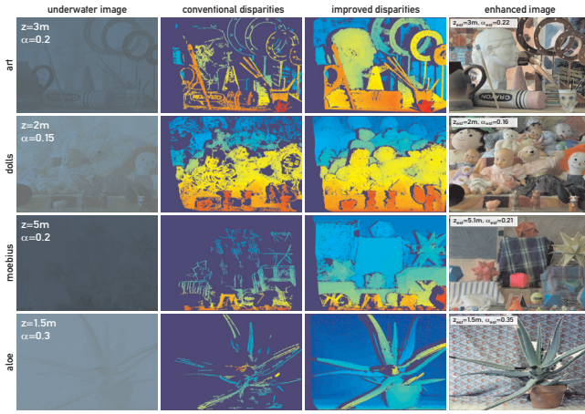
Fig. 5. Results on Middlebury Dataset. First column shows degraded underwater images, rendered with z = 3m , \alpha = 0.2 ( art ), z = 2m , \alpha = 0.15 ( dolls ), z = 5m , \alpha = 0.2 ( moebius ), z = 1.5m , \alpha = 0.3 ( aloe ). Second column shows their disparity maps. Third column shows the improved disparities (after step 1). Last column shows enhanced image (step 2).
